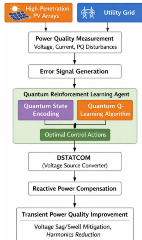
Figure 1. Quantum Reinforcement Learning-enabled DSTATCOM architecture
