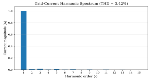
Figure 11. Harmonic spectrum of the injected grid current showing the total harmonic distortion of the grid current under ANN-based MPPT operation
