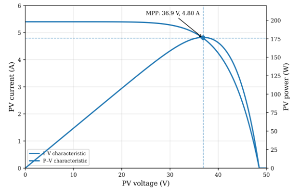
Figure 7. PV current–voltage and power–voltage characteristics under standard test conditions showing the maximum power point operating region Table 2 summarizes the dynamic MPPT performance at different irradiance and temperature levels. As irradiance increases from 650 to 1060 W/m 2 , the reported tracking time decreases from 0.082 to 0.055 s, while the tracking accuracy increases from 97.40% to 99.35%. Over the same operating range, the reported ripple index decreases from 0.021 to 0.013. At 1000 W/m 2 and 28.6°C, the controller achieves a tracking accuracy of 99.20%, a response time of 0.058 s, and a ripple index of 0.014. These results indicate improved convergence and reduced steady-state variation at higher irradiance levels under the investigated simulation conditions. The ripple values reported in Table 2 represent the normalized steady-state power oscillation around the maximum power point.
