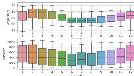
Figure 1. Monthly distribution of solar irradiance and ambient temperature measurements collected in Ngaoundéré (Cameroon) during the year 2023
