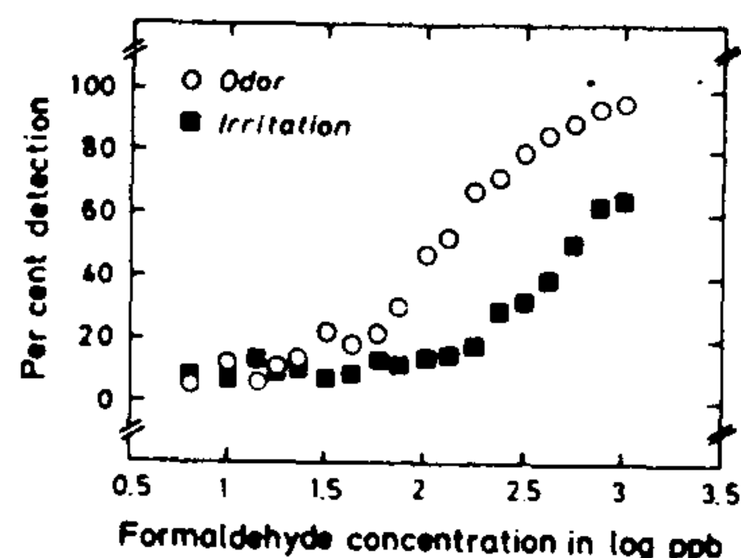
Fig. 7. Percent detections for the sensory classes odor (open circles) and irritation (filled squares) plotted against formaldehyde concentration in log ppb. The psychometric curves constitute the result for the group of 31 subjects.
