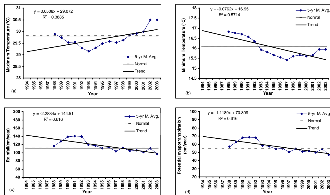
Fig. 4. Trend in 5-yearly moving average of maximum and minimum temperature, rainfall and potential evapotranspiration in the Balachaur watershed, Punjab, India during 1984 to 2003.
