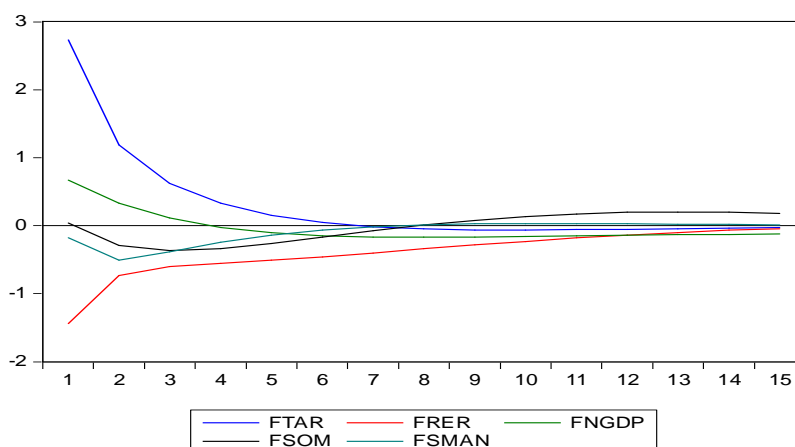
Response of FTAR to Generalized One S.D. Innovations
