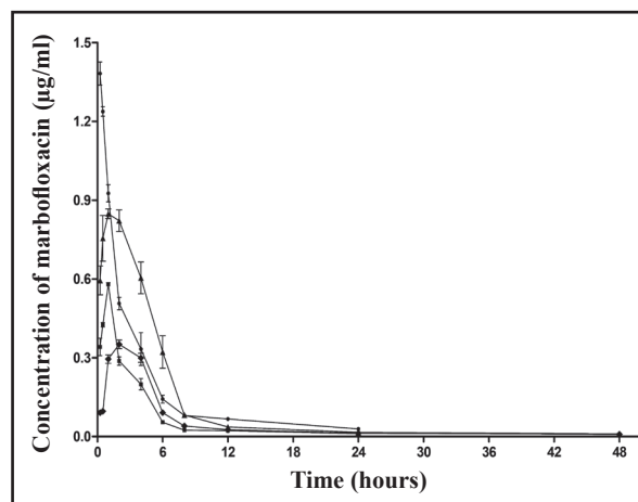
Figure 1. Marbofloxacin plasma and muscle concentration vs. time profiles, after intravenous and oral 2 mg/kg single dose in chickens (data as mean \pm SD). i.v plasma \blacksquare oral plasma \blacktriangle i.v muscle \bullet oral muscle \blacklozenge
