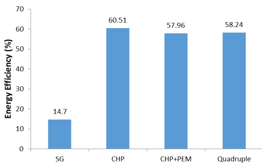
Figure 3. Advantages of cogeneration system in terms of energy efficiency
