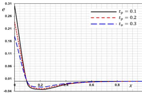
Figure 12. The effect of the pulse rises time of heat flux t_p on strain distributions e .
