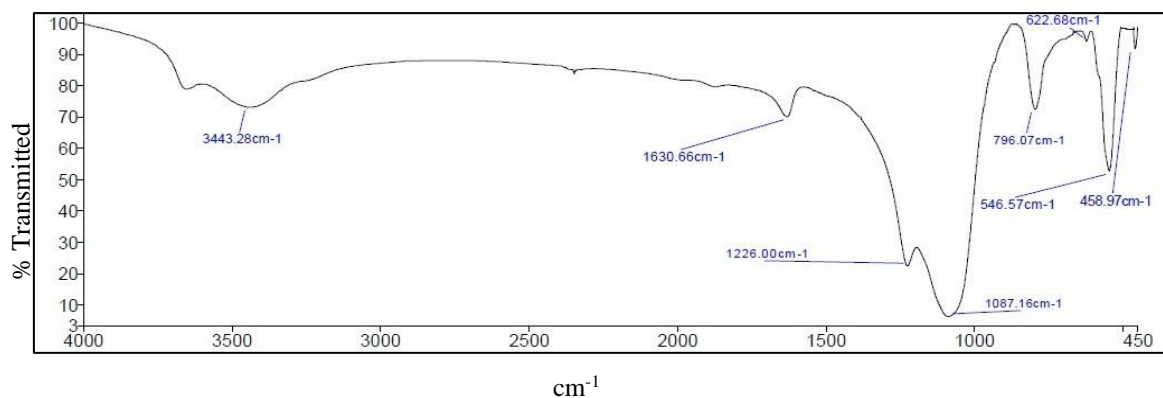
Fig. 4. The FT-IR spectrum of H-ZSM-5 zeolite between 4000-400 \text{cm}^{-1}
