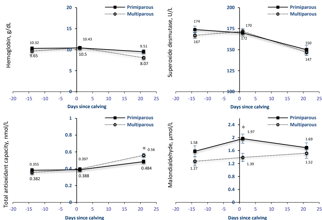
Figure 3. Blood antioxidant status of primiparous and multiparous dairy cows during transition period. Data were expressed as LSM with SE error bars. * P < 0.05 .
