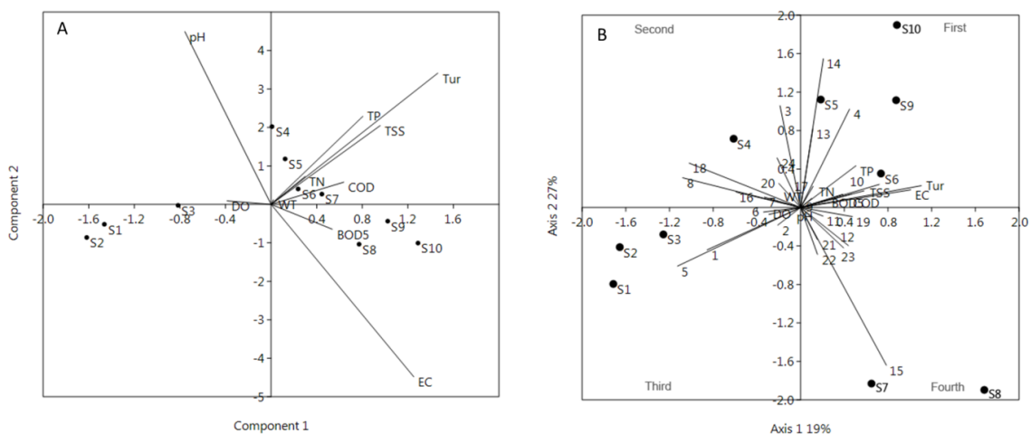
Fig. 5. Canonical correspondence analysis (CCA) diagram showing selected environmental variables and most frequently occurring diatom taxa in the ordination space of the first and second axes. Taxa codes correspond to those in Appendix 1.
