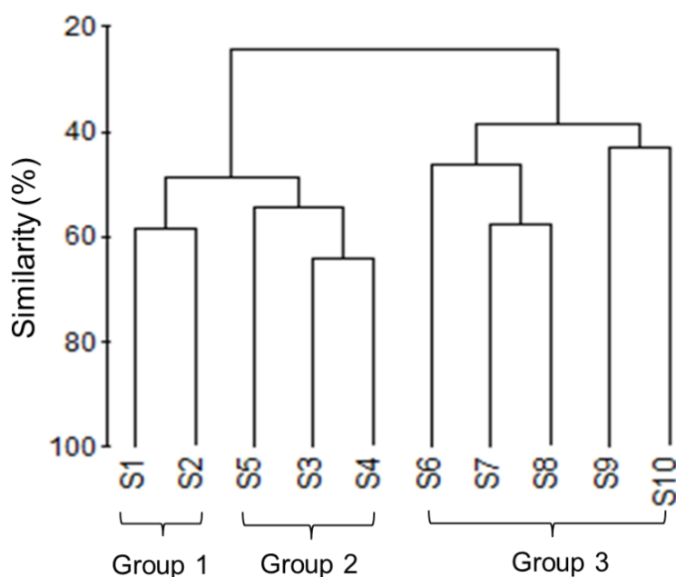
Fig. 4. Cluster analysis indicating the similarity of sites using diatom community structure and abundance at each site for dry and wet season.
