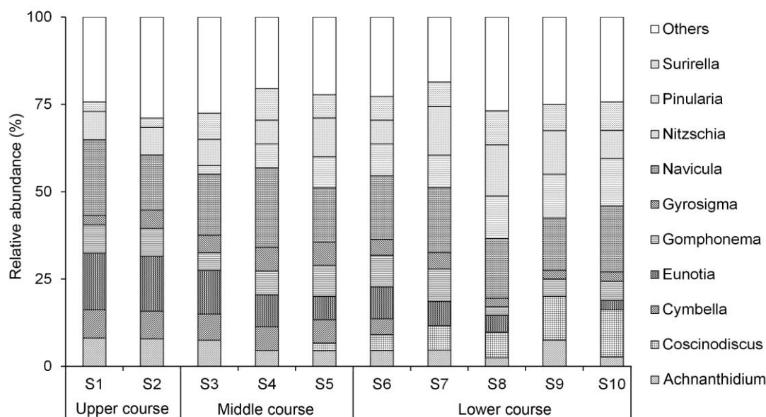
Fig. 2. Composition of 10 dominant genera at the sampling sites by combining samples of dry and wet season.
