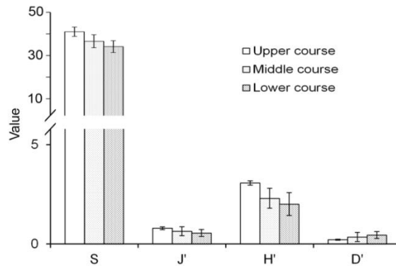
Fig. 3. Comparison of diversity indices (S, H' , J' , D' ) between upper course sites and lower course sites.
