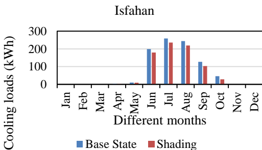
Figure 29. The graph comparing cooling loads of the base state and shading for Isfahan.
