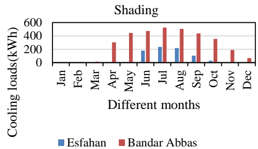
Figure 15. Monthly cooling loads for both studied cities in the state including smart shading.
