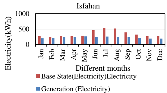
Figure 36. The graph of electricity consumption without solar generation (base state) and with solar generation for Isfahan.
