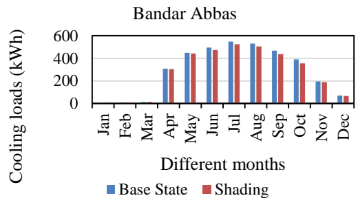
Figure 31. The graph comparing cooling loads of base state and shading for Bandar Abbas.
