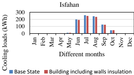
Figure 17. The graph comparing cooling loads of base state and walls insulation for Isfahan.
