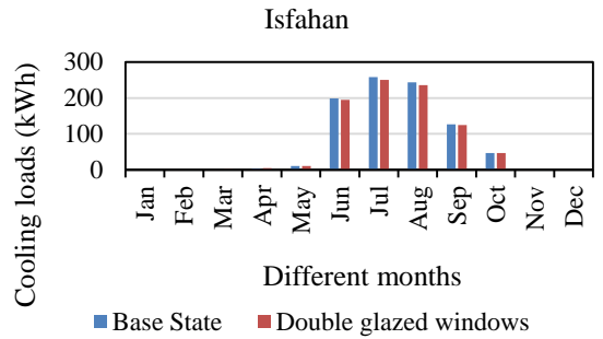
Figure 25. The graph comparing cooling loads of the base state and double glazed for Isfahan.
