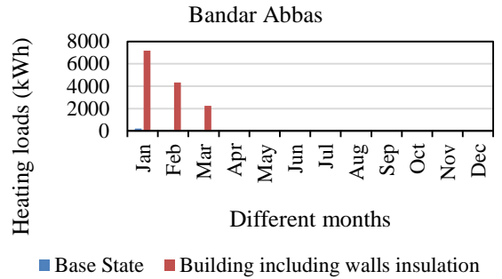
Figure 20. The graph comparing heating loads of base state and walls insulation for Bandar Abbas.
