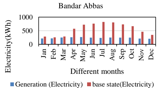
Figure 37. The graph of electricity consumption without solar generation (base state) and with solar generation for Bandar Abbas.
