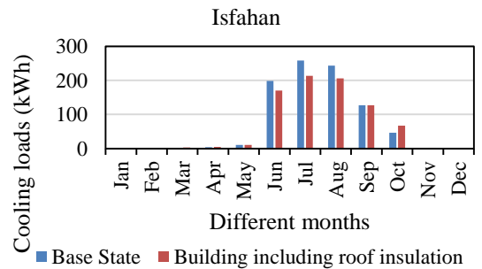
Figure 21. The graph comparing cooling loads of base state and ceiling insulation for Isfahan.
