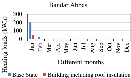
Figure 24. The graph comparing heating loads of base state and ceiling insulation for Bandar Abbas.
