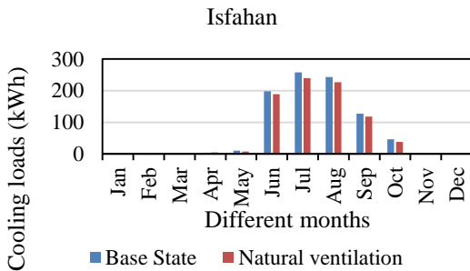
Figure 33. The graph comparing cooling loads of base state and natural ventilation for Isfahan. The solar generated electricity due to installed photovoltaic panels is presented in figures 34 and 35 for Isfahan and Bandar Abbas, respectively.
