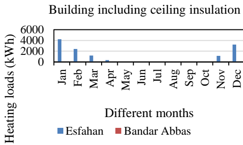
Figure 12. Monthly heating loads for both studied cities in the state that ceiling insulation included.
