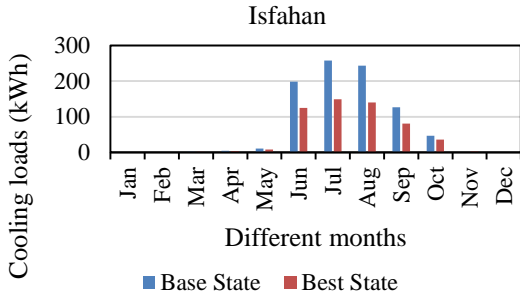
Figure 38. Comparative graph for cooling loads of the building in Isfahan: the base state and the most optimized state.
