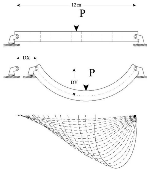
Fig. 10. Simple support beam deformation curve
