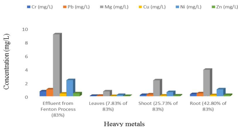
Fig. 2. Heavy metal removal efficiency after Fenton process
