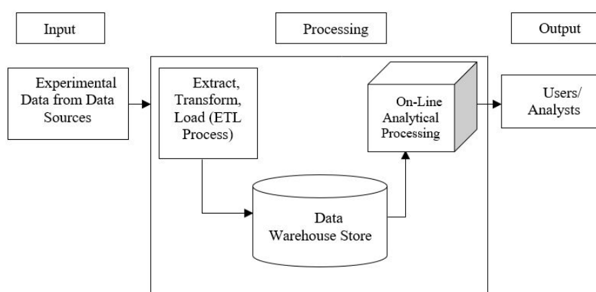
Figure 1. OLAP and Data Warehouse Framework
