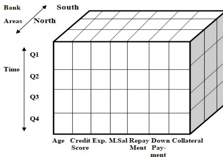
Figure 3. Loan Management Data Cube
