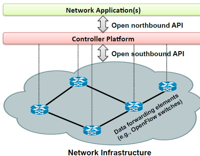
Figure 1. Structure of an SDN
