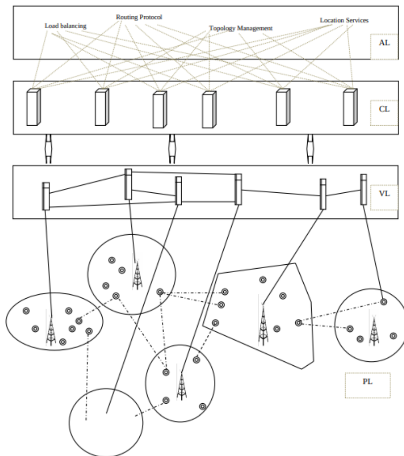
Figure 5. Network Framework
