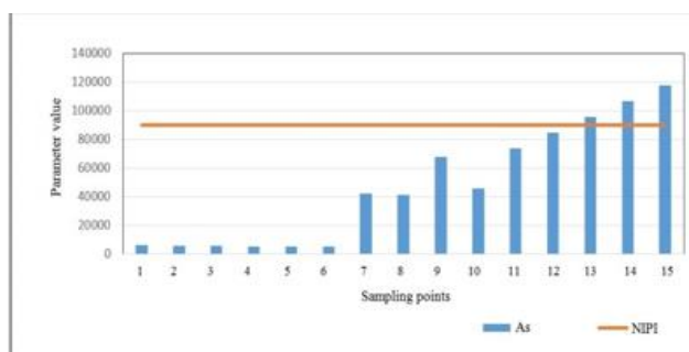
f- NIPI and As values
