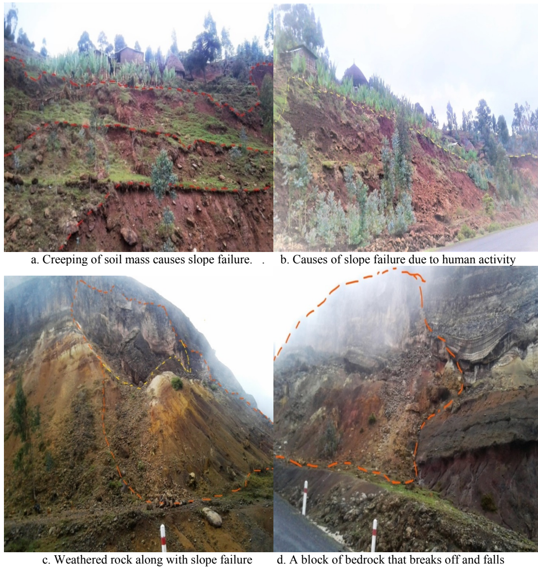
Figure 3. Sample photo that shows failure Rock-soil slope along road corridor
