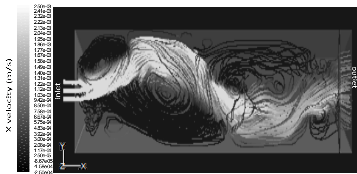
Fig. 4. Path lines colored by velocity magnitude (m/s) in the equalization pond
