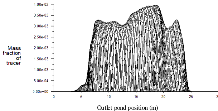
Fig. 5. Mass fraction tracer as a function of the outlet position in the equalization lagoon after 4.5h of the application of the tracer pulse
