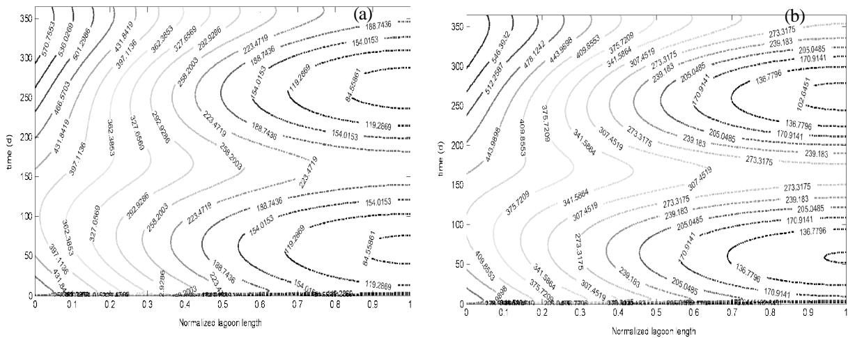
Fig. 9. Contours of S_C along the aerated lagoon length during a year (365d): (a) current operation and (b) increasing Q in 12.5%.
