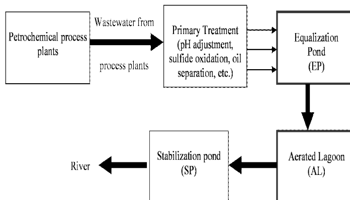
Fig. 1. Petrochemical wastewater treatment system
