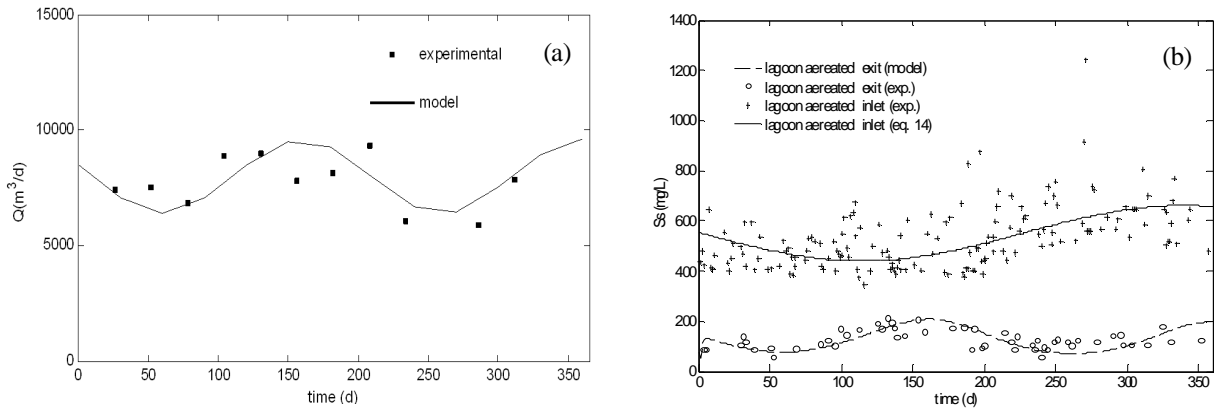
Fig. 7. (a) Flow rate ( Q ) and (b) substrate ( COD ) fluctuations ( S_C ), as a function of time
