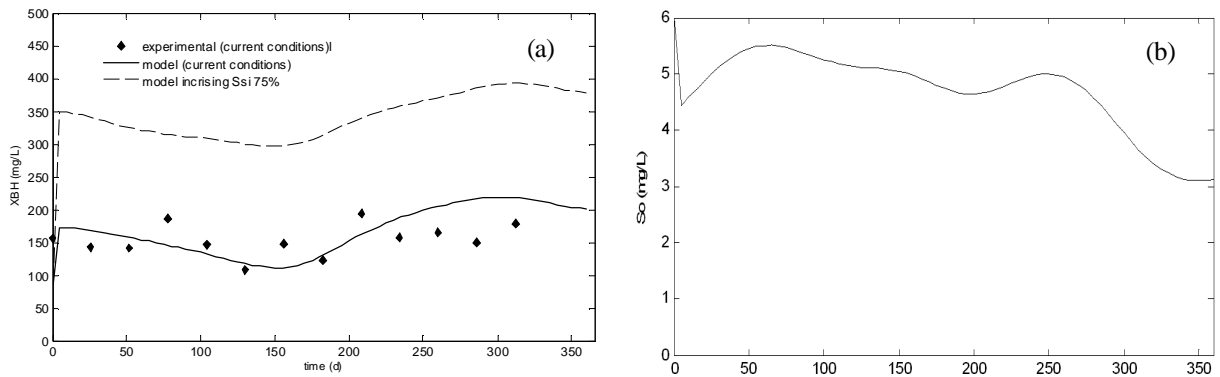
Fig. 8. Variation of (a) X_{BH} and (b) dissolved oxygen ( S_O ) in the lagoon effluent, as a function of time.
