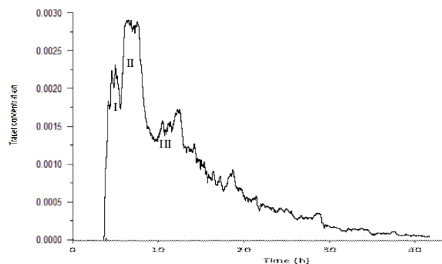
Fig. 6. Tracer concentration as a function of time at the pond outlet
