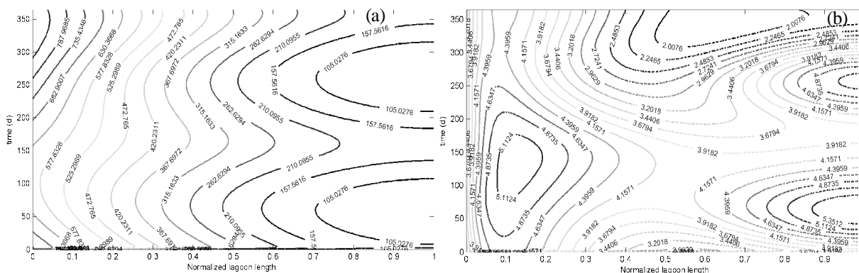
Fig. 10. Contours of (a) S_s and (b) S_0 along the aerated lagoon length during an operation of 365 d, increasing the influent substrate concentration ( S_{Si} ) in 75% and aeration in 50%
