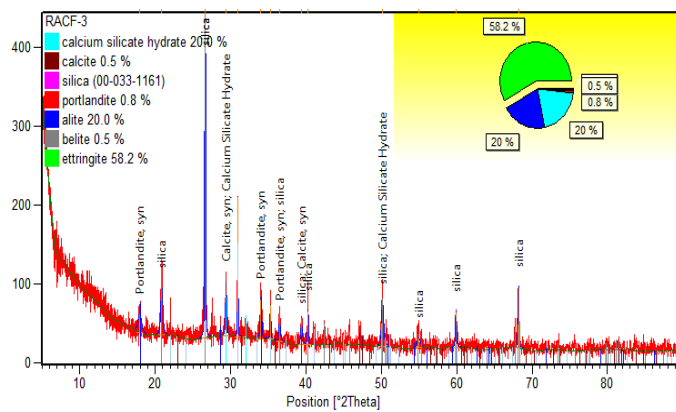
Fig. 4. XRD patterns for RAC-F-3 mix
