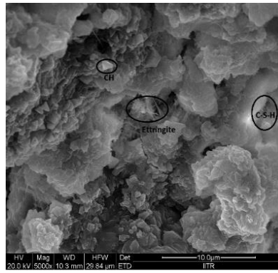
(c) Fig. 5. SEM images for RAC-BA: a) RAC-BA-1; b) RAC-BA-2; and c) RAC-BA-3
