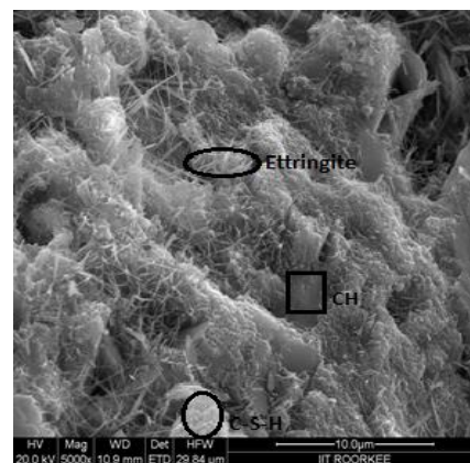
Fig. 2. SEM image for RAC mix
