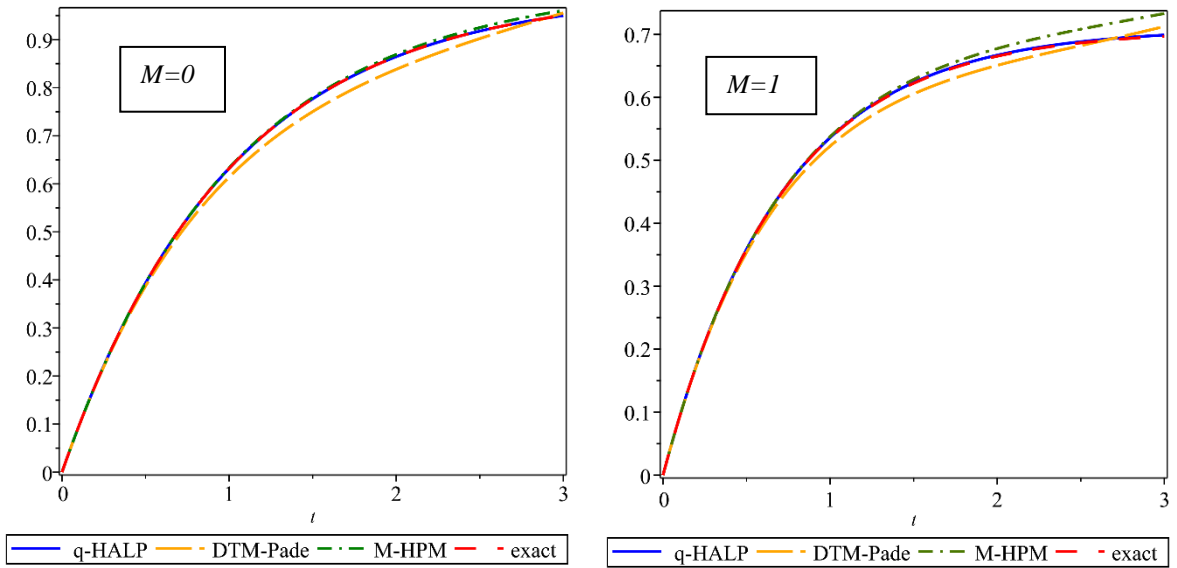
Fig-4: Compression between q- HALP , M-HPM and DTM- Padé with exact where \beta = 1
