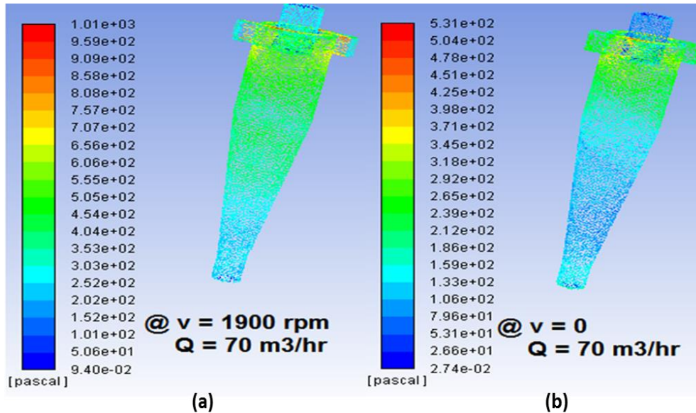
Fig. 10. Pressure vectors at flow rate of 70 \text{ m}^3/\text{hr} and the rotation speed of (a) 1900 rpm and (b) 0 rpm
