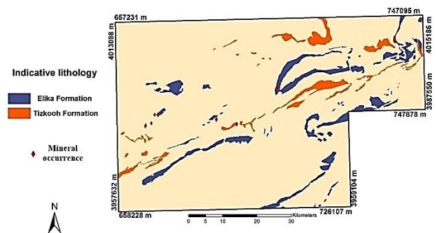
Figure 2. The indicator lithostratigraphic features of MVT-fluorite mineralization, Elika formation: limestone and dolomite rocks with the age of Triassic. Tizkooh formation: Orbitolina limestone with the age of lower Cretaceous.
