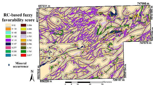
Figure 7. Mineral prospectivity model for the MVT-fluorite deposit, generated using the RC -based fuzzy logic modelling with fuzzy sum operator.
