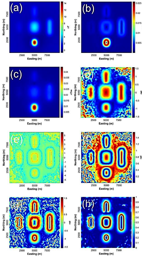
Fig 5. a) Magnetic anomaly map of the synthetic model with upward continuation of 200 m, b) THD, c) AS, d) TA, e) HTA, f) TM, g) TAHG, h) LTHD.
