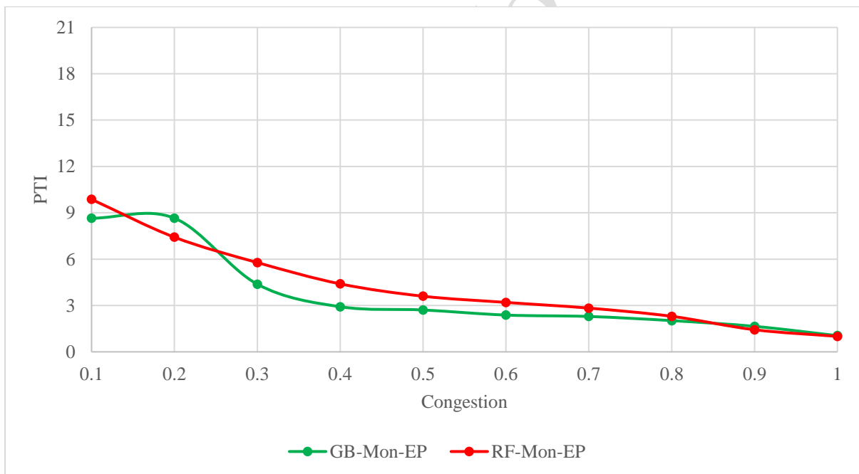
Fig 2 (b): Comparison between GB and RF modeling results- Monday evening peak
