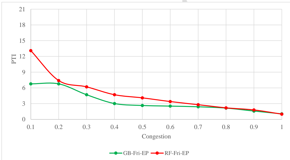
Fig 6 (b): Comparison between GB and RF modeling results- Friday evening peak
