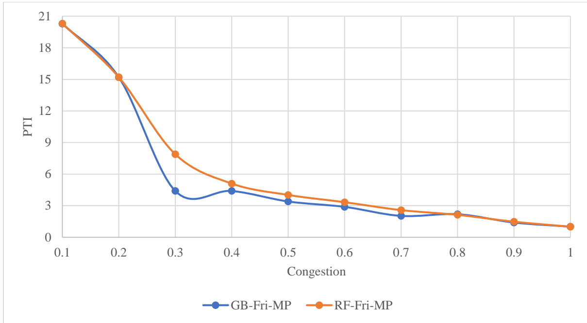
Fig 6 (a): Comparison between GB and RF modeling results- Friday morning peak
