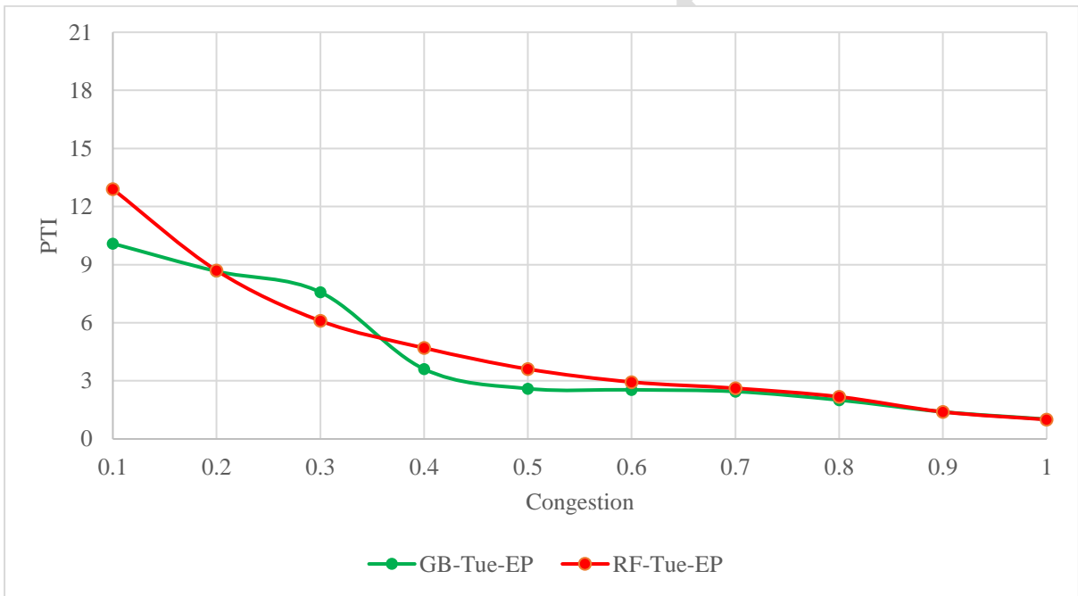
Fig 3 (b): Comparison between GB and RF modeling results- Tuesday evening peak
