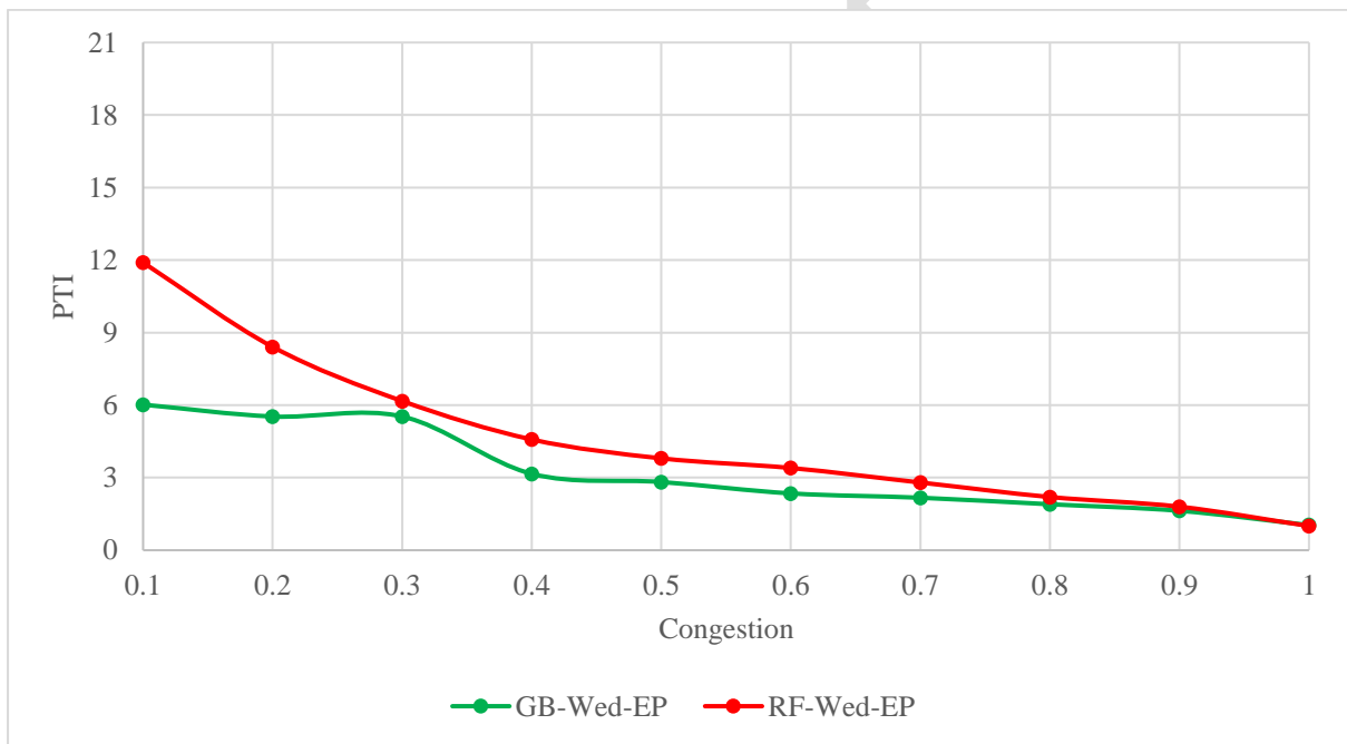
Fig 4 (b): Comparison between GB and RF modeling results- Wednesday evening peak
