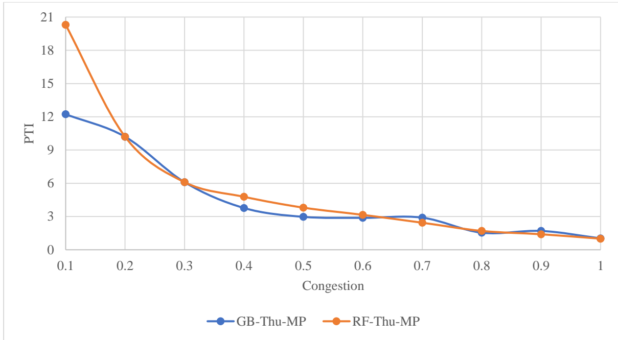
Fig 5 (a): Comparison between GB and RF modeling results- Thursday morning peak
