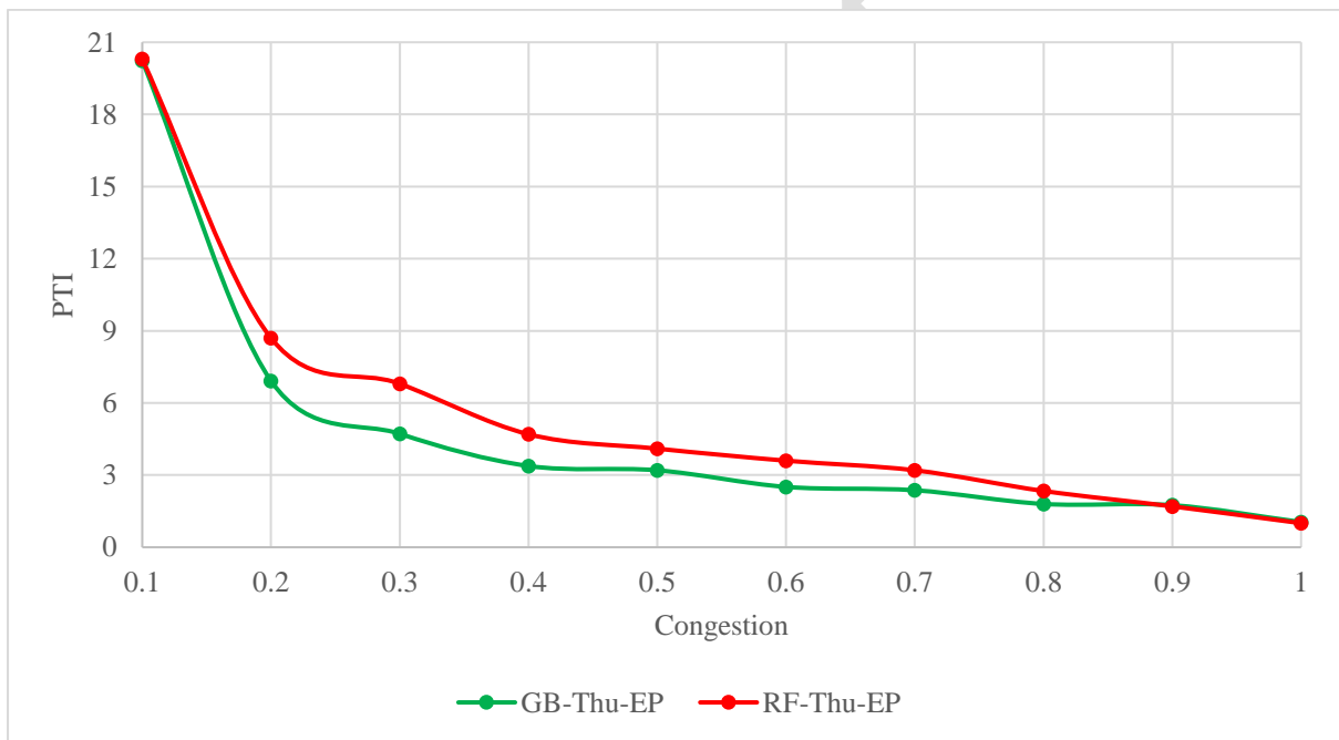
Fig 5 (b): Comparison between GB and RF modeling results- Thursday evening peak
