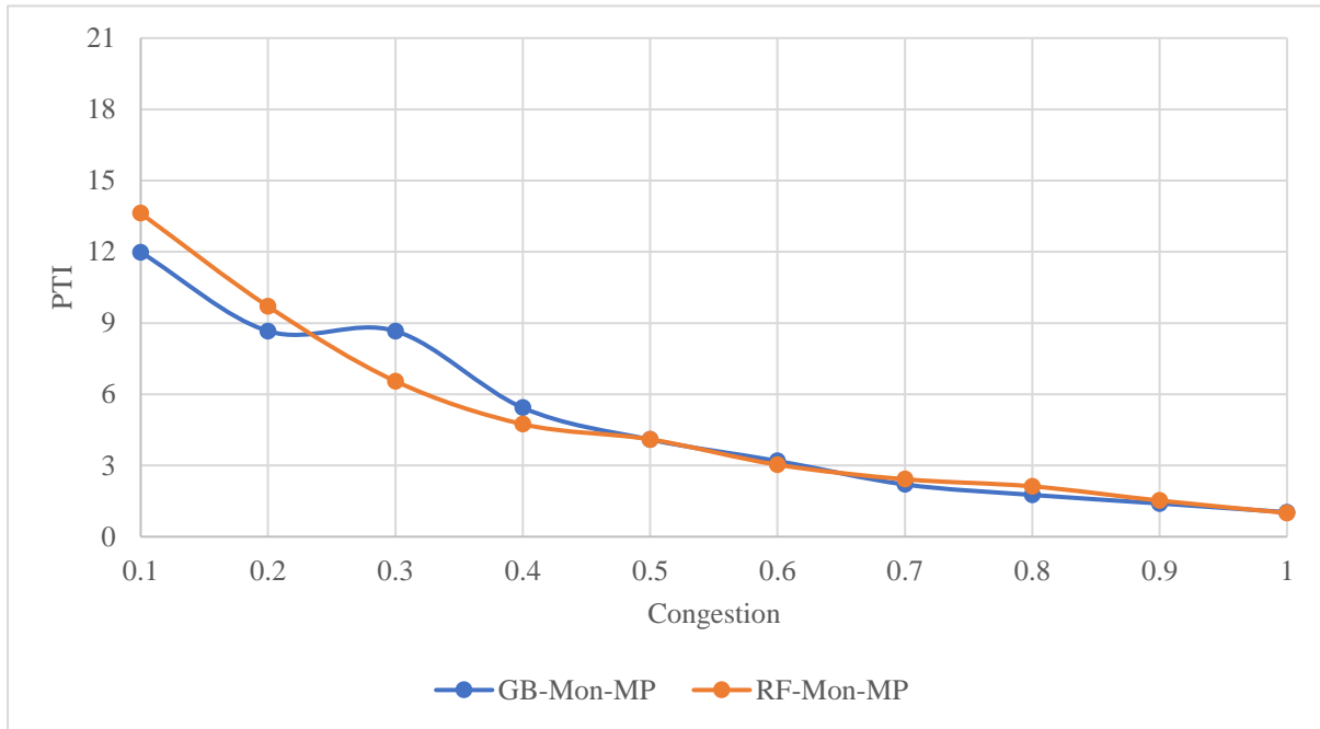
Fig 2 (a): Comparison between GB and RF modeling results- Monday morning peak
