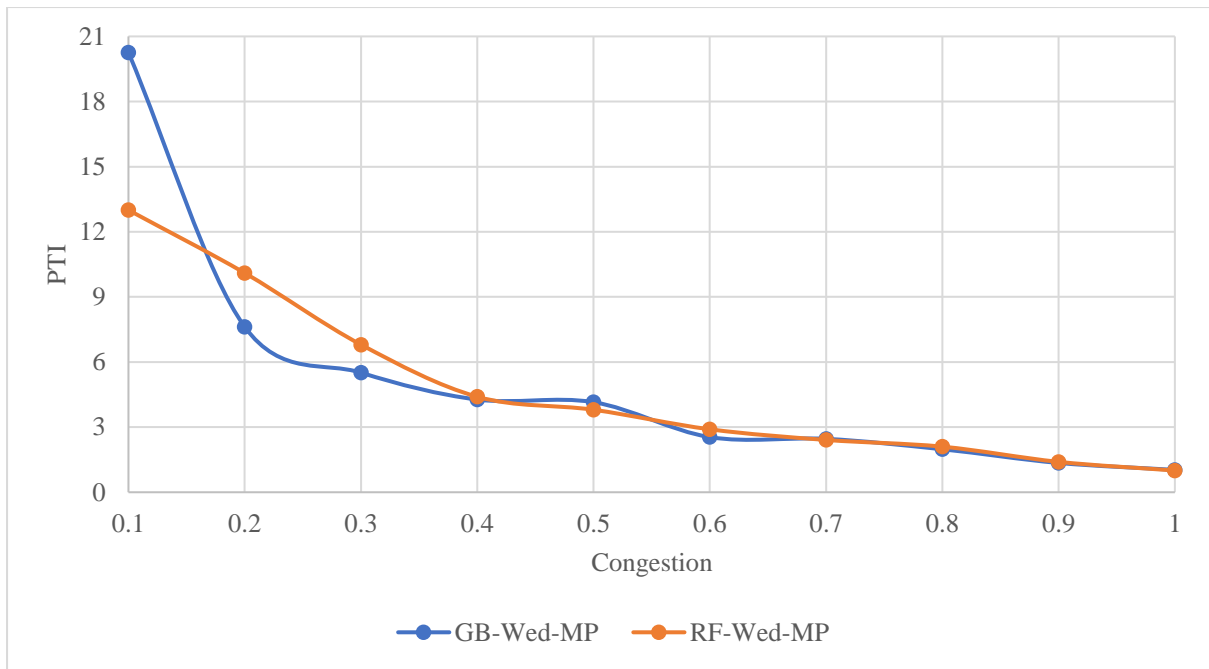
Fig 4 (a): Comparison between GB and RF modeling results- Wednesday morning peak
