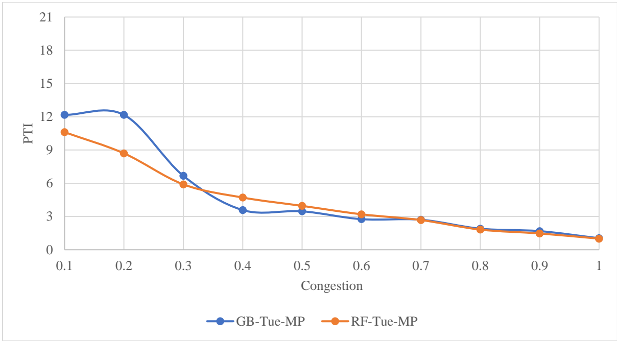
Fig 3 (a): Comparison between GB and RF modeling results- Tuesday morning peak
