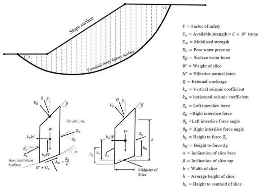
Fig. 1. Division of potential sliding mass into slices
