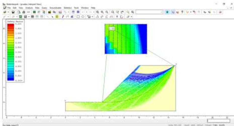
Fig. 5. The FOS from SLIDE
