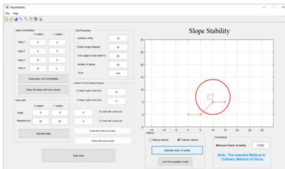
Fig. 6. The FOS from the Matla code
