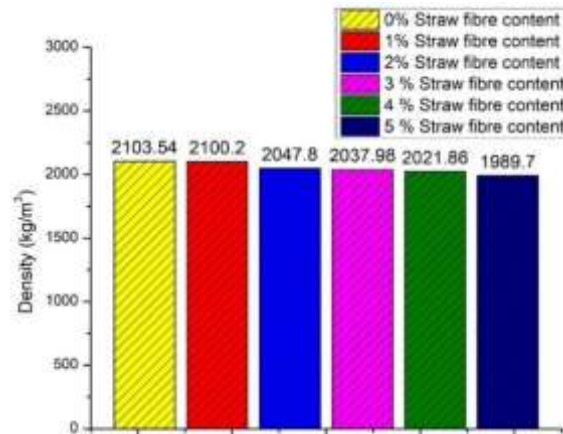
Fig. 3. Density of CSC with straw fibre content (%) at 28 days of curing
