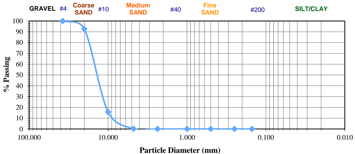
Fig. 1. Particle size distribution curve for coconut shell aggregate
