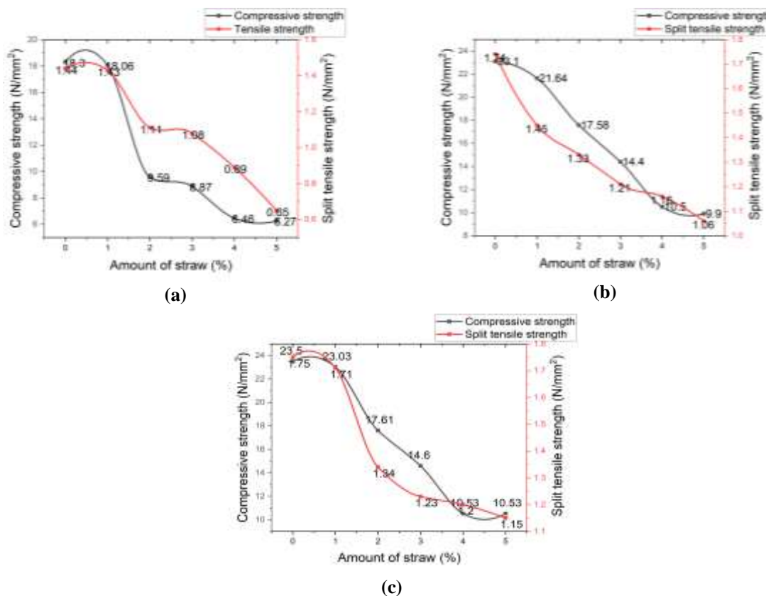
Fig. 5. Relationship between compressive strength and split tensile of CSC with straw fibre content (%) at: a) 7 days; b) 28 days; and c) 56 days of curing
