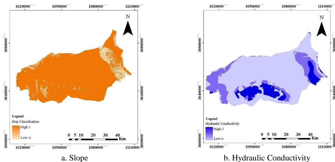
Fig. 6. Thematic layers classified by Fuzzy membership degree in the soft formation of the Shamil-Takht watershed
