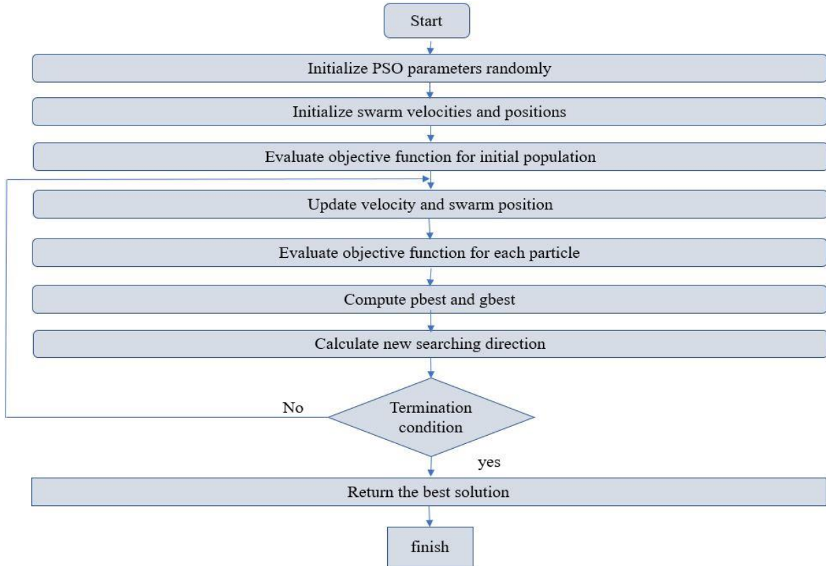
Fig 2. PSO algorithm
