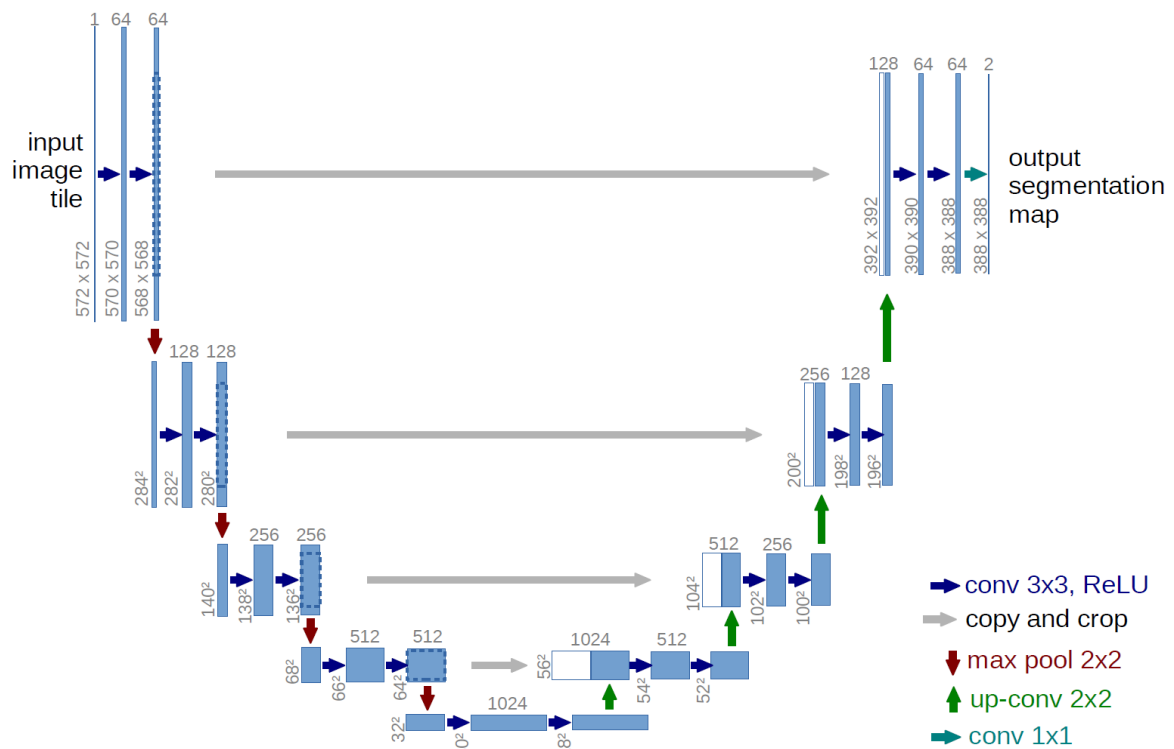
Fig 3. U-net structure[38]
