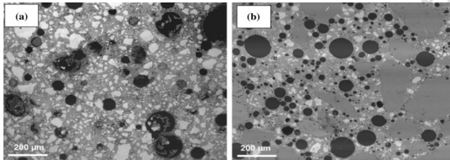
Figure 2 For resistance to frost, CC with a SAP and b SAP-created air gaps(Wong,2018)
