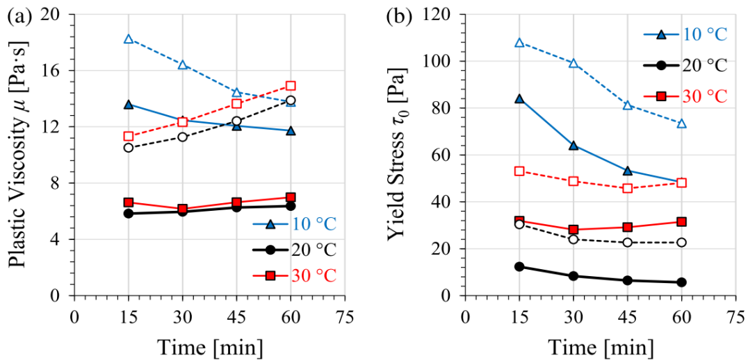
Figure 1: Effects of temperature on plastic viscosity and yield stress
