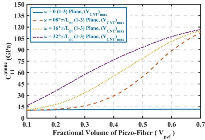
Fig. 8: Effective elastic property of PMNC ( C_{11}^{pmnc} ) with CNTs oriented along 1-3 plane.
