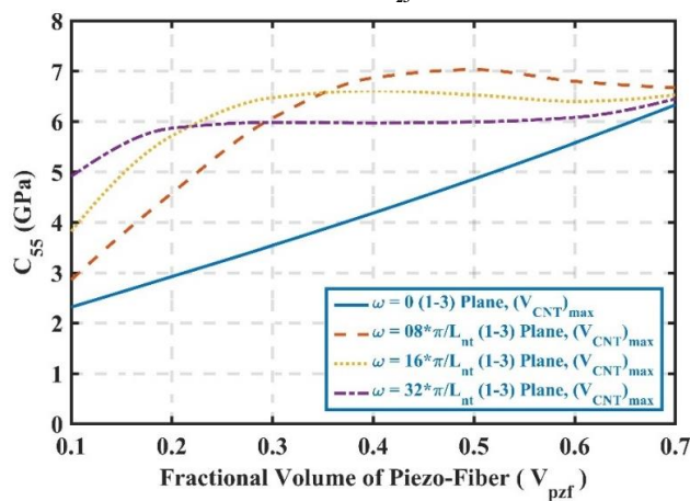
Fig 16: Effective elastic property of SPFFRC ( C_{55} ) with CNTs oriented along 1-3 plane.
