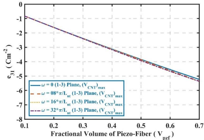
Fig 19: Effective Piezoelectric Coefficient e_{31} of the overall SPFFRC with CNTs oriented along 1-3 plane.
