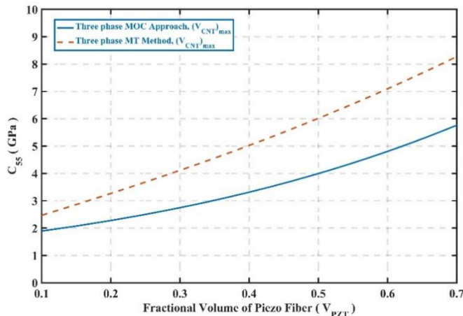
Fig 31: Comparison of effective property C_{55} estimated using MOC approach and MT method.
