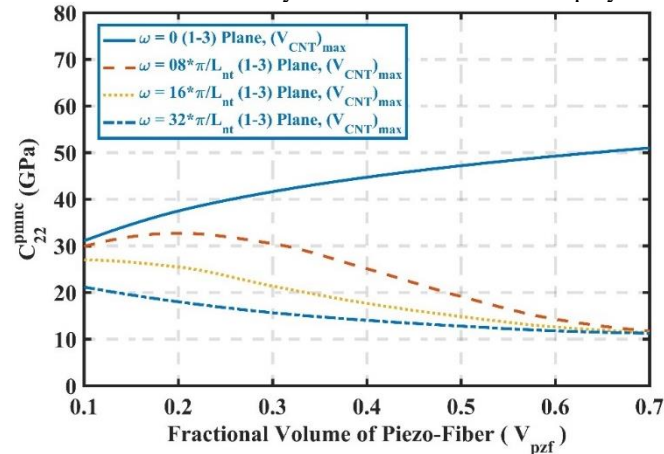
Fig 9: Effective elastic property of PMNC ( C_{22}^{pmnc} ) with CNTs oriented along 1-3 plane.
