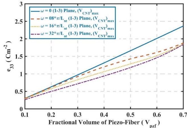
Fig 20: Effective Piezoelectric Coefficient e_{33} of the overall SPFFRC with CNTs oriented along 1-3 plane.
