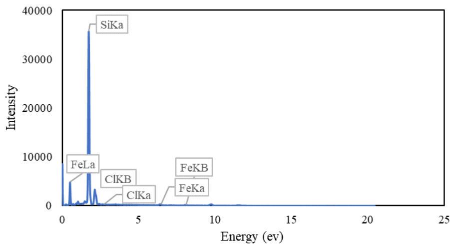
Fig. 8. EDX analysis of orange silica gel-based RHA and \text{FeCl}_3 \cdot 6\text{H}_2\text{O}
