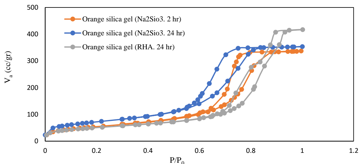
Fig. 5. N_2 adsorption-desorption of orange silica gel-based commercial sodium silicate and RHA
