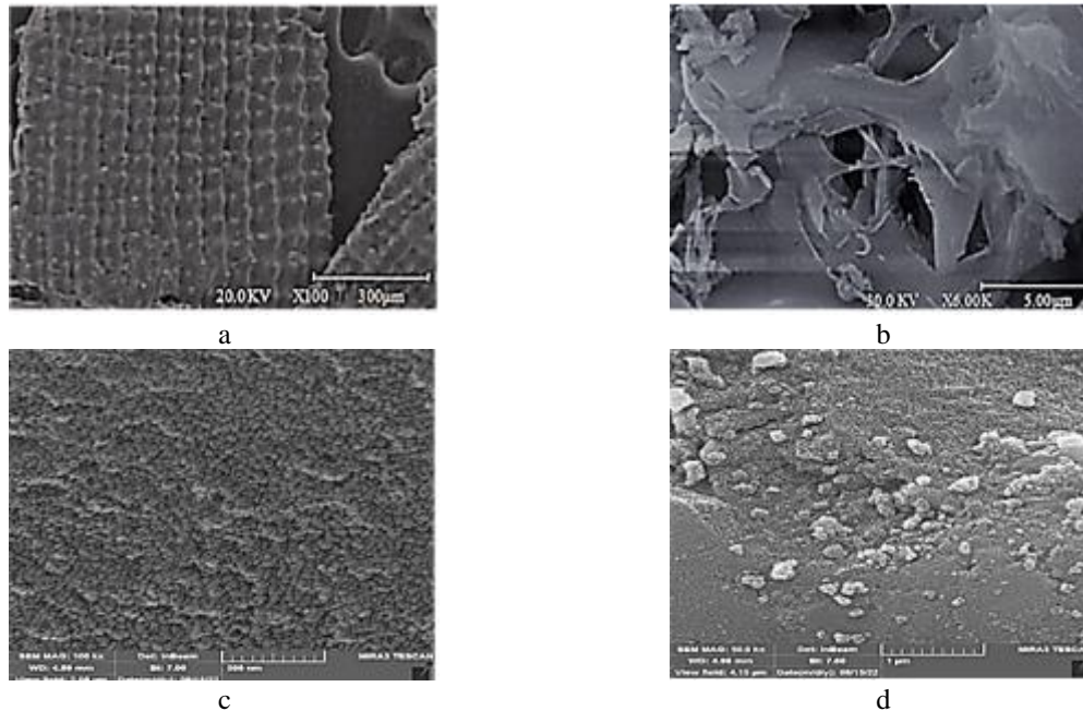
Fig. 6. FESEM images of a) RH, b) RHA, orange silica gel based on RHA c) 500 nm d) 1 micrometer
