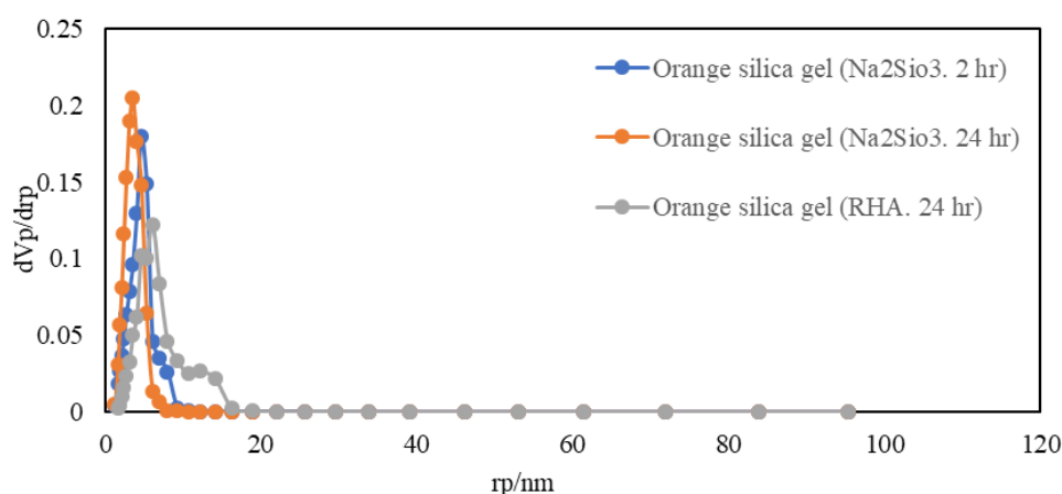
Fig. 6. Pore size distribution of orange silica gel-based commercial sodium silicate and RHA
