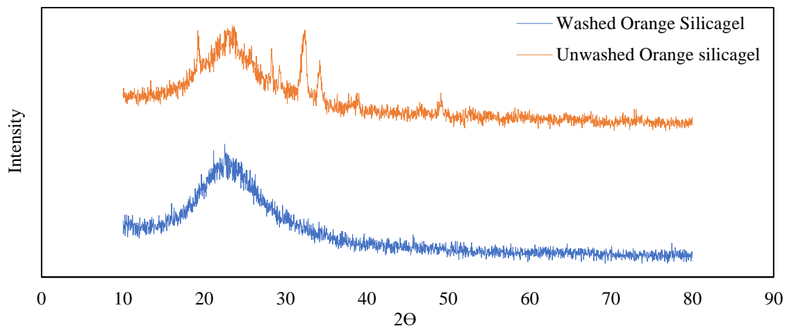
Fig. 4. XRD pattern of unwashed and washed orange silica gel based on RHA
