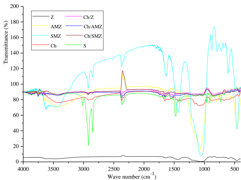
Fig. 3. FTIR spectra of natural zeolite, chitosan, Ch/ Z, AMZ, SMZ, Ch/AMZ and Ch/ SMZ
