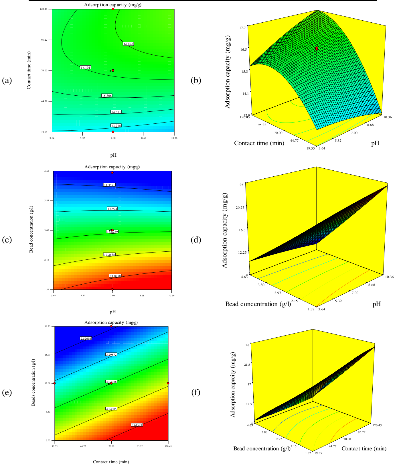
Fig. 7. Response surface 3D plot and contour plot for the interaction of two parameters on adsorption capacity when the other parameters at the middle level
