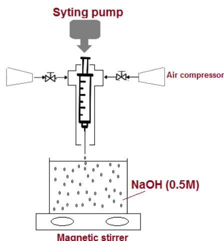
Fig. 1. Experimental set-up for production of chitosan/zeolite beads
