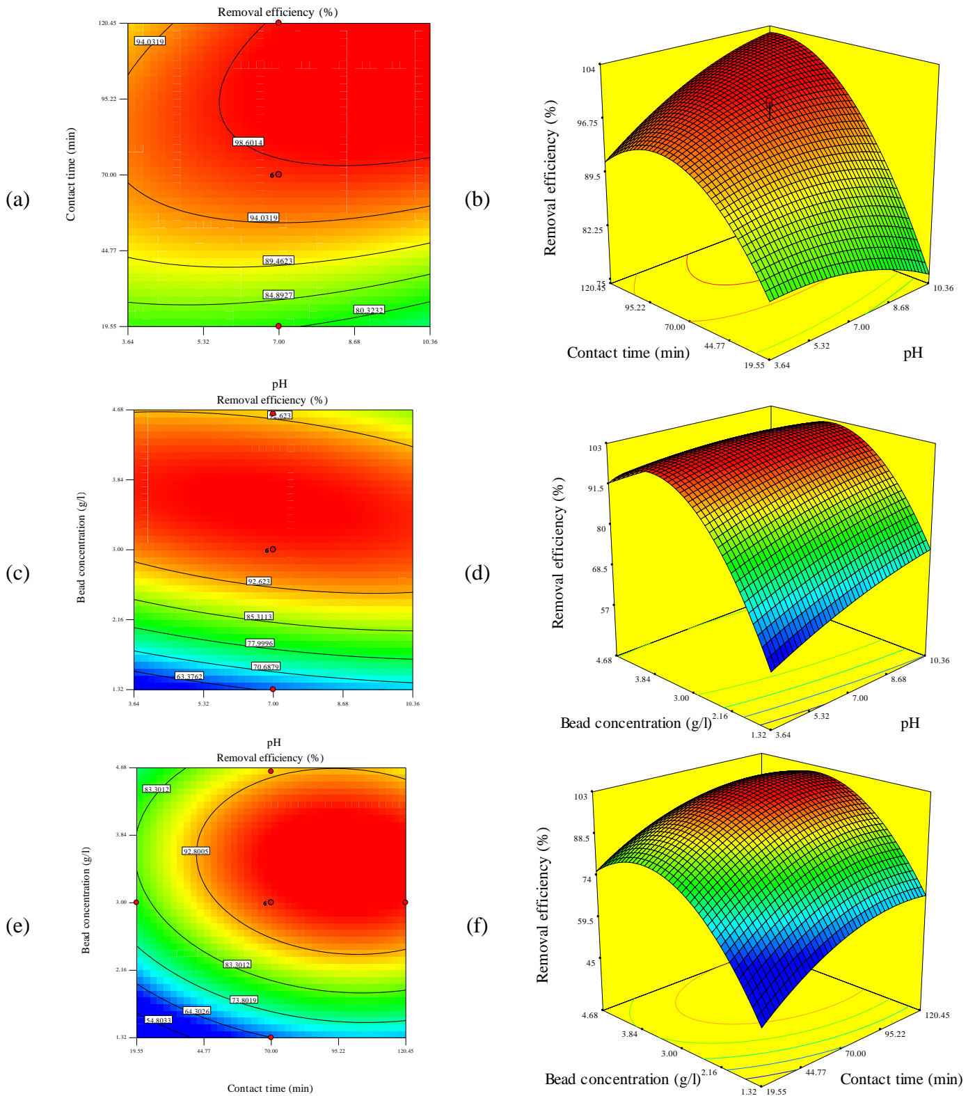
Fig. 6. Response surface 3D plot and contour plot for the interaction of two parameters on the removal efficiency when the other parameters at the middle level
