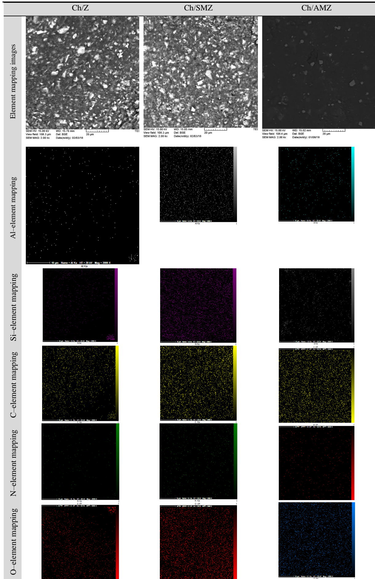
Fig. 5. Element mapping results for Ch/Z, Ch/SMZ, and Ch/AMZ
