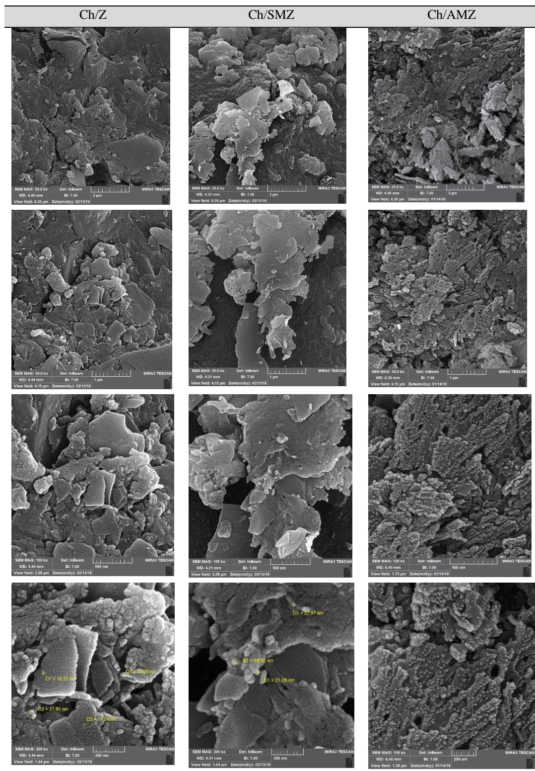
Fig. 4. Scanning electron micrographs of (FE-SEM) for Ch/Z, Ch/SMZ, and Ch/AMZ
