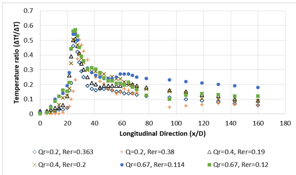
Fig. 8. Dilution of the plume center temperature ratios for the single-port submerged diffuser obstructed by fixed vanes at H=2 .
