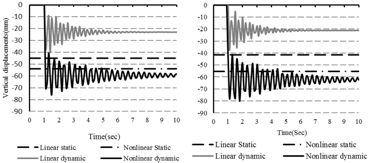
(c) Sudden removal of the column C13.
